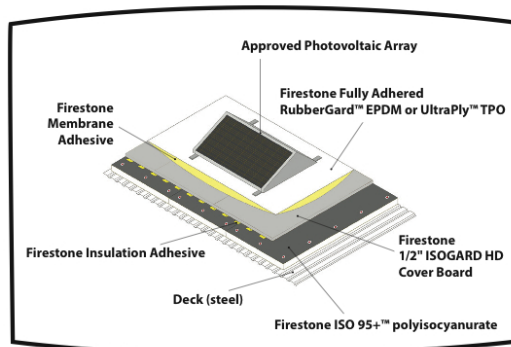
TPO System with PV
